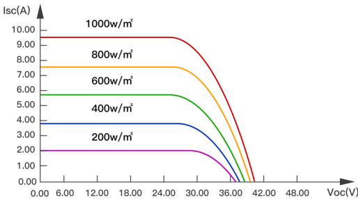
I-V Curves of PV module MS2 M-60 at various solar irradiance 95
