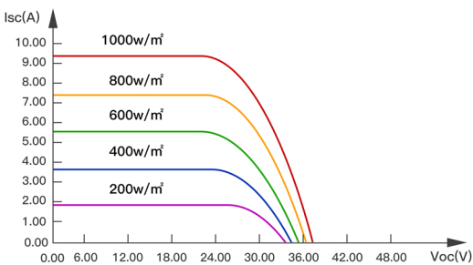
I-V Curves of PV module MS26 B-60 at various solar irradiance
