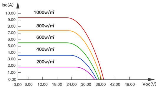
I-V Curves of PV module MS265P-60 at various solar irradiance
